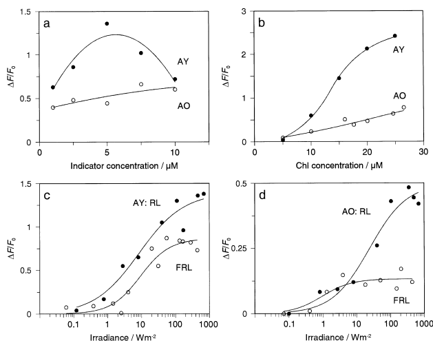
Fig. 3. Characterization of light-induced fluorescence changes of the \Delta pH indicators Acridine yellow and Acridine orange in dependence of indicator concentration (a), chlorophyll a concentration (b) or irradiance (c,d), respectively. Chlorophyll a concentration in a,c,d was about 15 \mu M; indicator concentration in b–d was 5 \mu M; irradiance in a,b was 500 \text{W m}^{-2} . For the AY signal the dark–light transition was used, for the AO signal the light–dark transition was used (see Fig. 2d,f).
